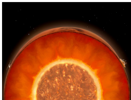
Artist's view of the internal structure of Mars. The molten silicate layer is visible at the base of the mantle.
